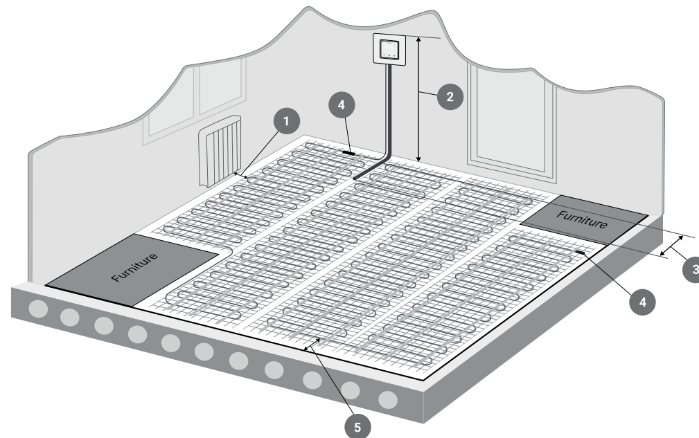
Fig.1 The example of laying the heating mat
